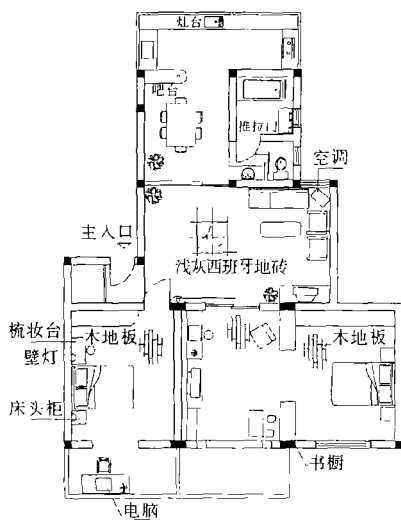
图 4 中间卧室作书房户型平面布置 Fig.4 Plane space of middle house as a study
